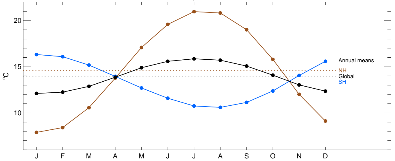
CRU absolute temperature 1961-1990 mean
